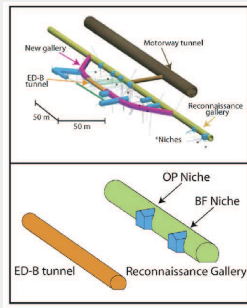
Figure 3.28: Relative location of the ED-B tunnel to the Motorway tunnel and Reconnaissance gallery (Corkum and Martin, 2007a).
