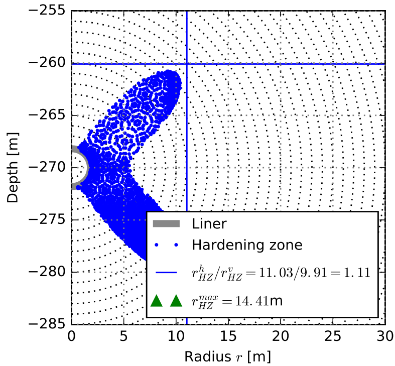
Figure 3.33: Gaussian integration points showing the extent of the Hardening zone (HZ) ( c = 3.6 MPa, \phi = 24.0^\circ ).
