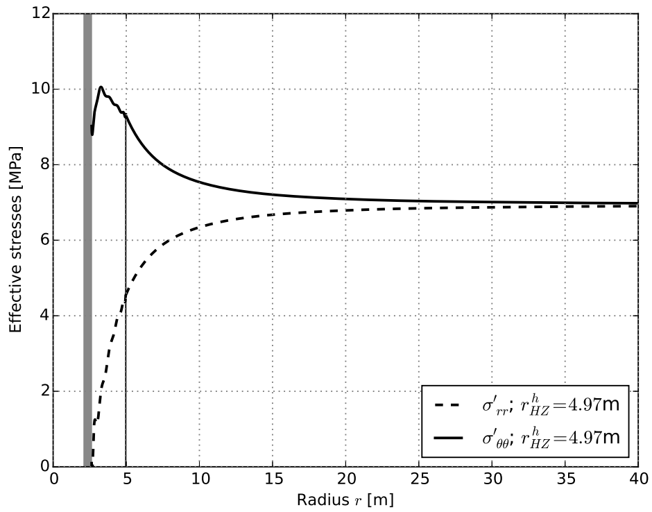
Figure 3.22: Effective radial and tangential stress distributions in the horizontal direction.
