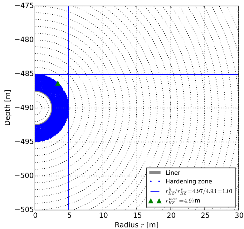
Figure 3.24: Gaussian integration points showing the extent of the Hardening Zone (HZ).
